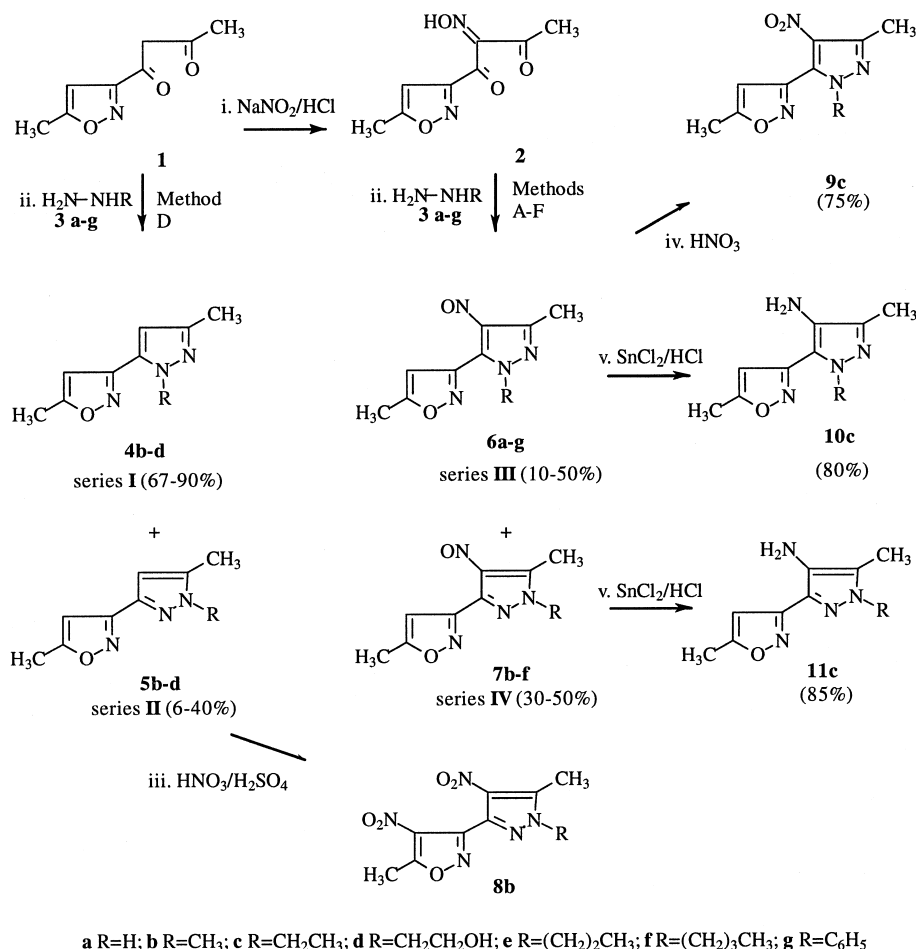
Scheme 1. (i) NaNO 2 /HCl in water at rt; (ii) method A: water at rt; B: dichloromethane at rt for 10 min; C ethanol at 0 °C to rt; D: ethanol at reflux for 1 h; E: water/OH - at rt; F: acetic acid at reflux for 1 h; (iii) H 2 SO 4 /HNO 3 at rt for 3 h; (iv) HNO 3 on ice bath in 5 h; (v) SnCl 2 /HCl concd at 0 °C.
