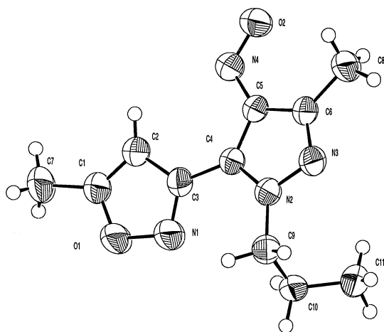
Figure 1. Perspective view of the molecular structure of 6e . Thermal ellipsoids are drawn at the 50% probability level.
