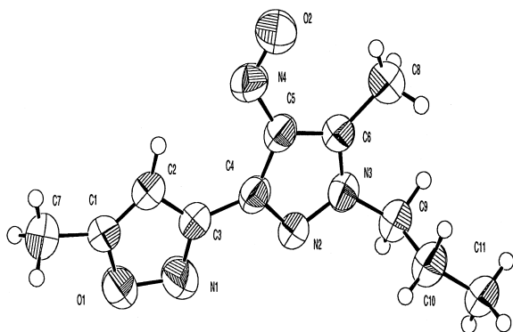
Figure 2. Perspective view of the molecular structure of 7e . Thermal ellipsoids are drawn at the 50% probability level.
